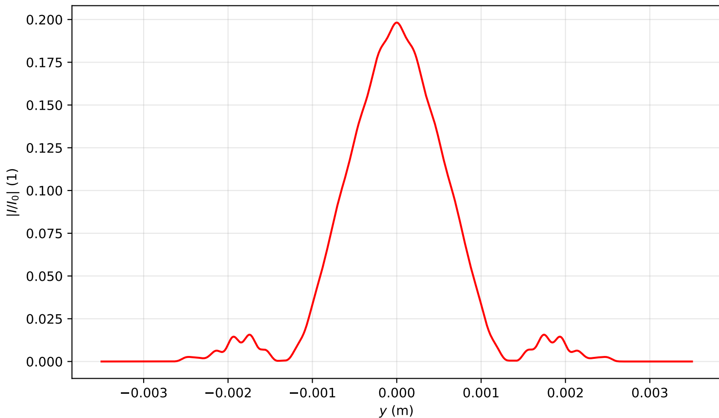
Intensity profile I(x=0, y, z=1.433)/I_0 , Pin=2.0Pcr, artificial time
